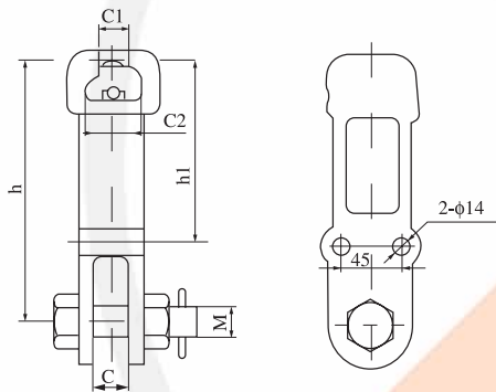
Socket-Clevis (Type WS)
