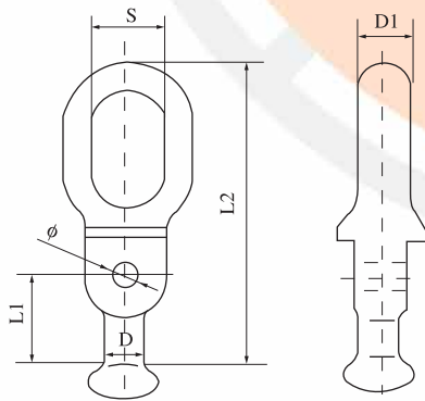
Ball Eyes (Parallel Type)
