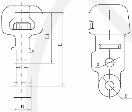
Socket Clevis (Type W)
